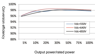
Efficiency curve
