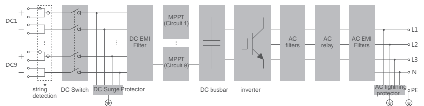
Circuit block diagram
