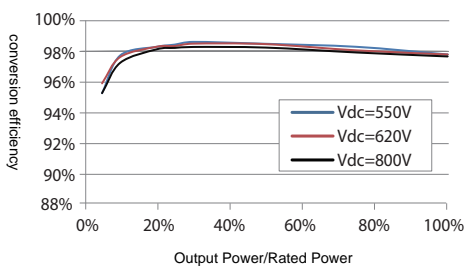
Efficiency Curve
