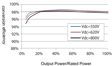
Efficiency Curve
