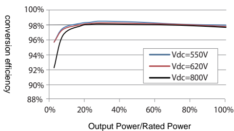
Efficiency Curve
