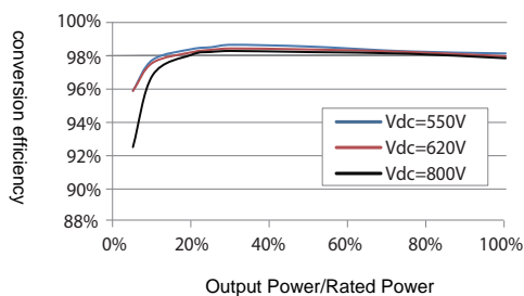
Efficiency Curve
