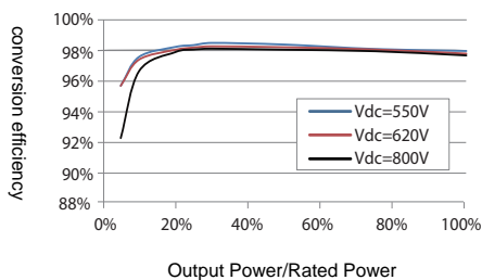
Efficiency Curve
